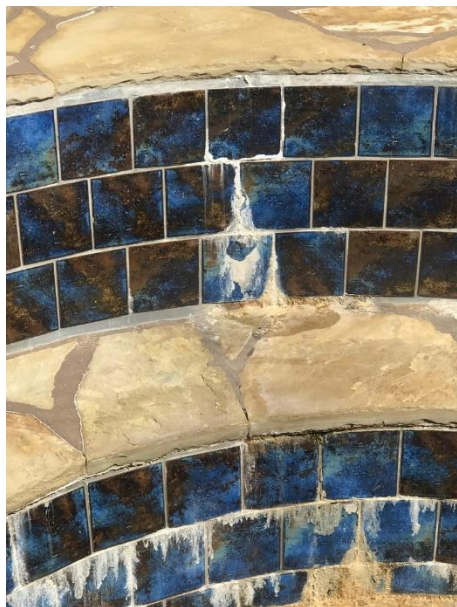
PHOTO: Failure to waterproof. Water pushes through concrete, creating efflorescence on the other side. In this case, a recessed firepit in the middle of the pool.
